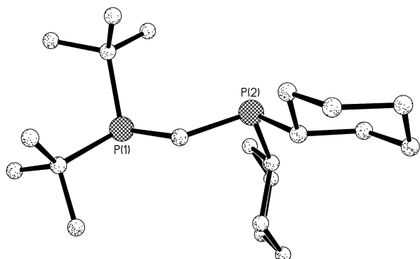
Fig. 7 Calculated minimum geometry for 3 (RHF/6-31G**). Hydrogen atoms have been omitted for clarity.
